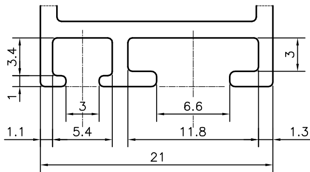
DETAIL OF "A" SCALE 3:1
