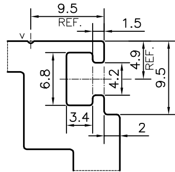
DETAIL OF "D" SCALE 2:1
