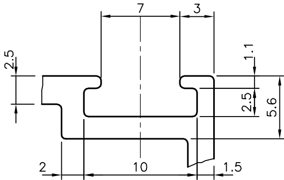
DETAIL OF "B" SCALE 3:1
