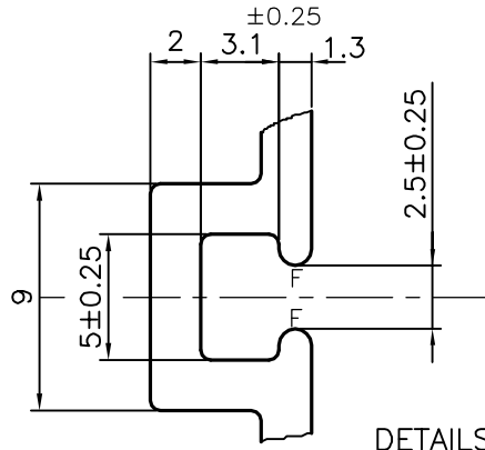
DETAILS OF "A" SCALE 3:1
