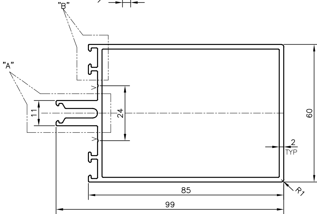
DETAIL "A" SCALE 3:1
