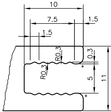
DETAIL OF "A" SCALE 3:1
