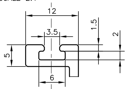
DETAIL 'B'
