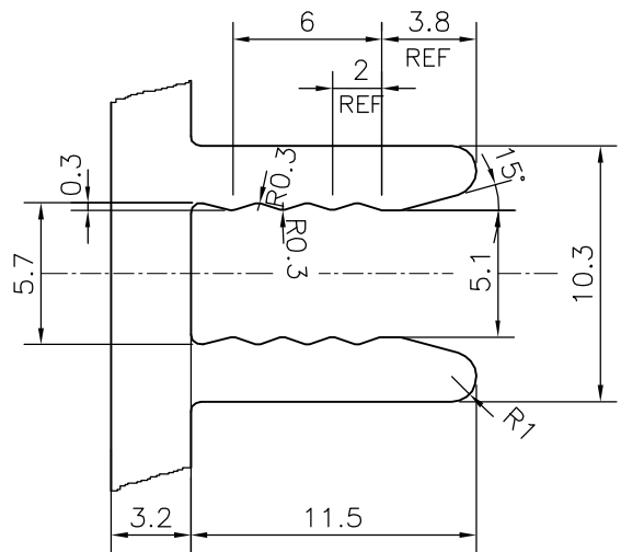
DETAIL OF "A" SCALE 3:1
