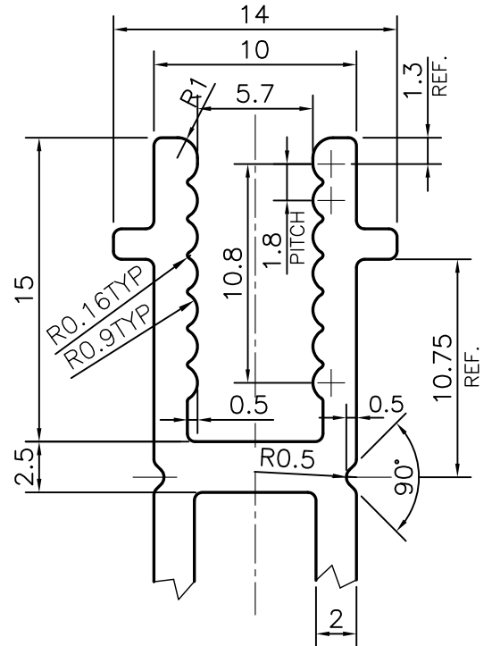
DETAIL OF "A" SCALE 3:1
