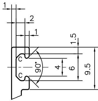
DETAIL OF "B" SCALE 2:1
