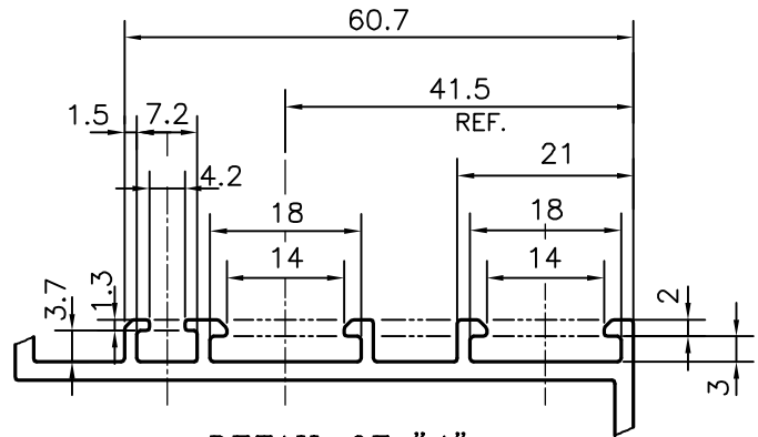
DETAIL OF "A" SCALE 1:1
