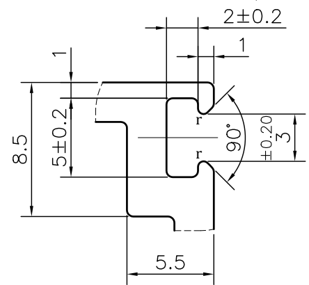
DETAIL B SCALE 3:1
