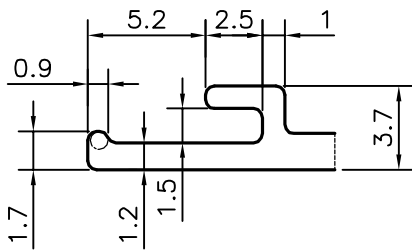
DETAIL OF "A" SCALE 3:1
