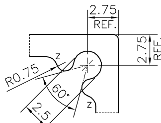
DETAIL OF "A" SCALE 3:1
