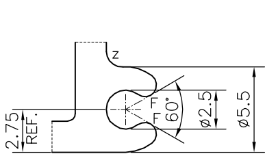
DETAIL OF "A" SCALE 3:1
