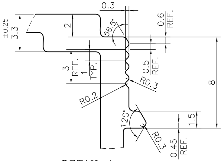
DETAIL A SCALE 5:1
