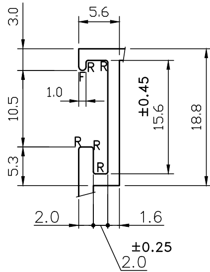
DETAIL AT- B
