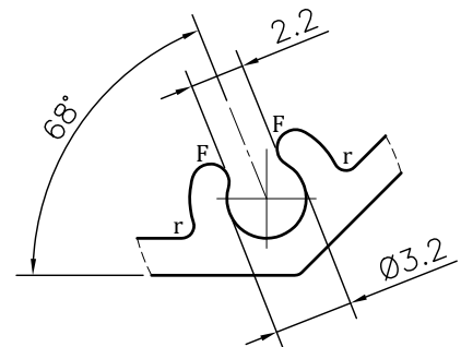
DETAIL B SCALE 3:1
