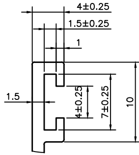
DETAIL AT=A
