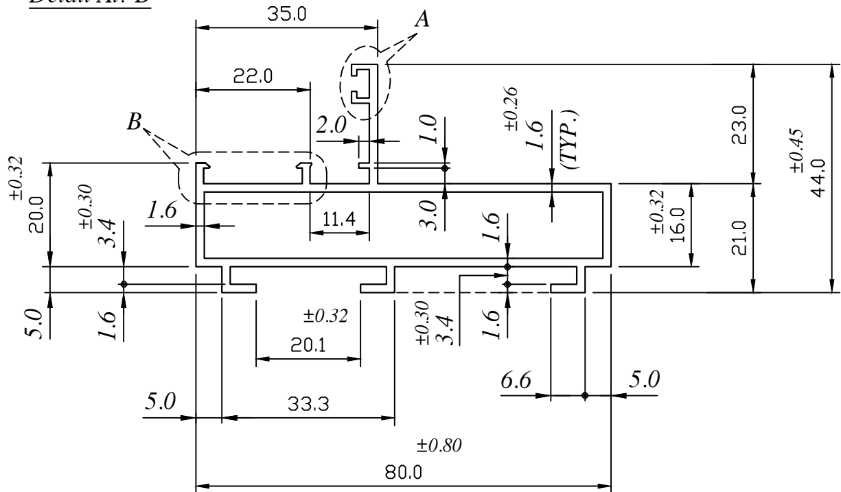
Detail At:-B
