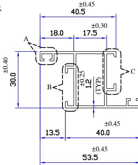
DETAIL AT-C
