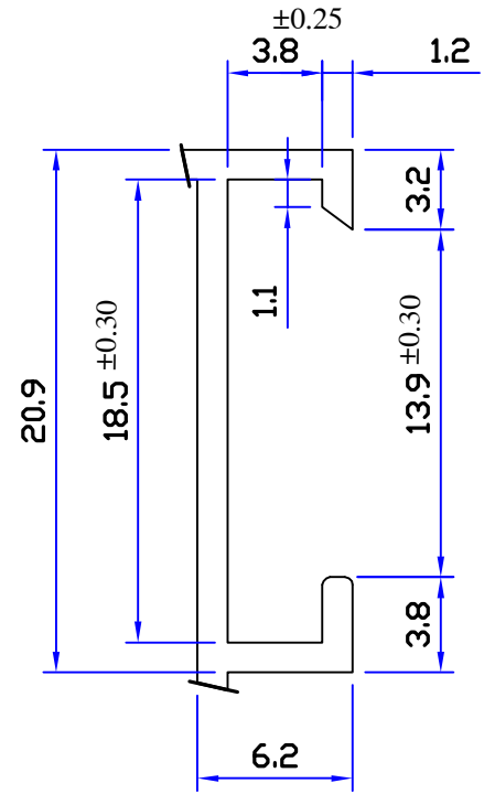
DETAIL AT-C
