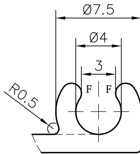
DETAIL-A SCALE 3:1
