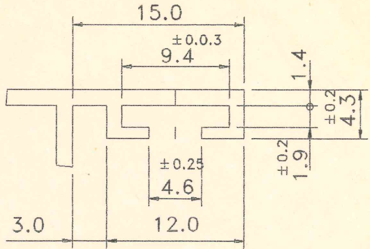
DETAIL AT-A
