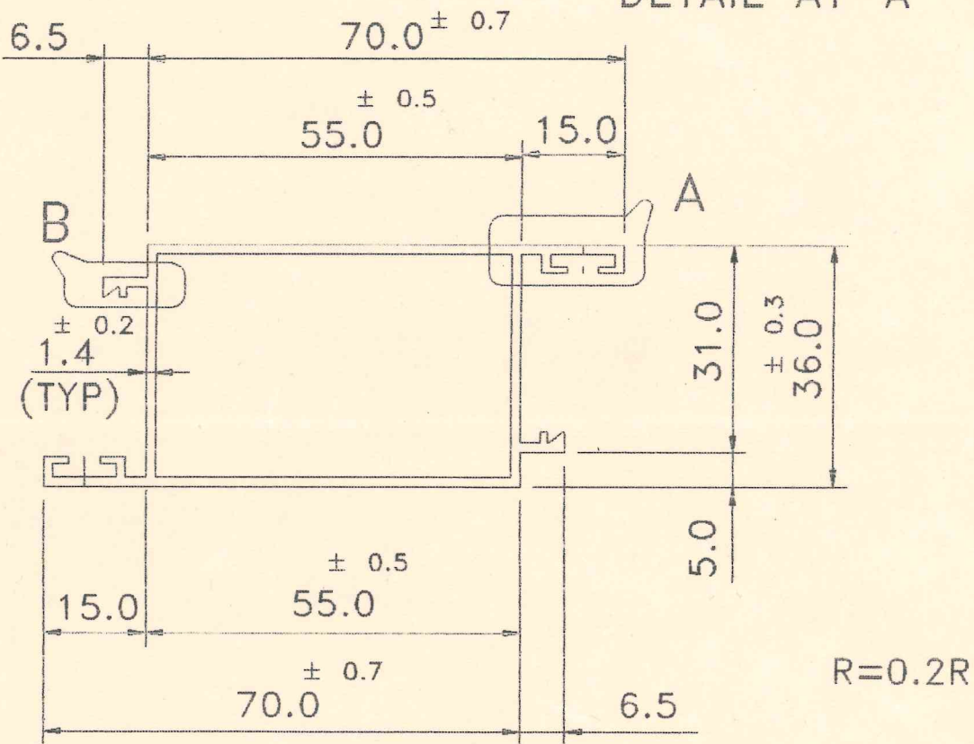
DETAIL AT-A
