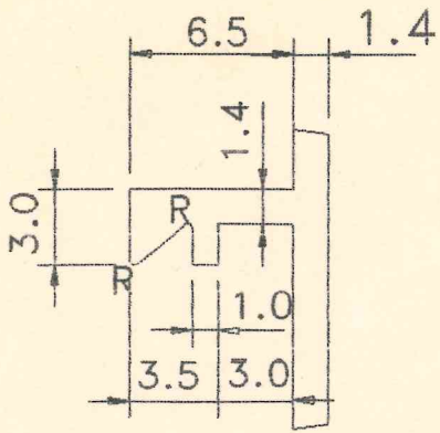
DETAIL AT-B
