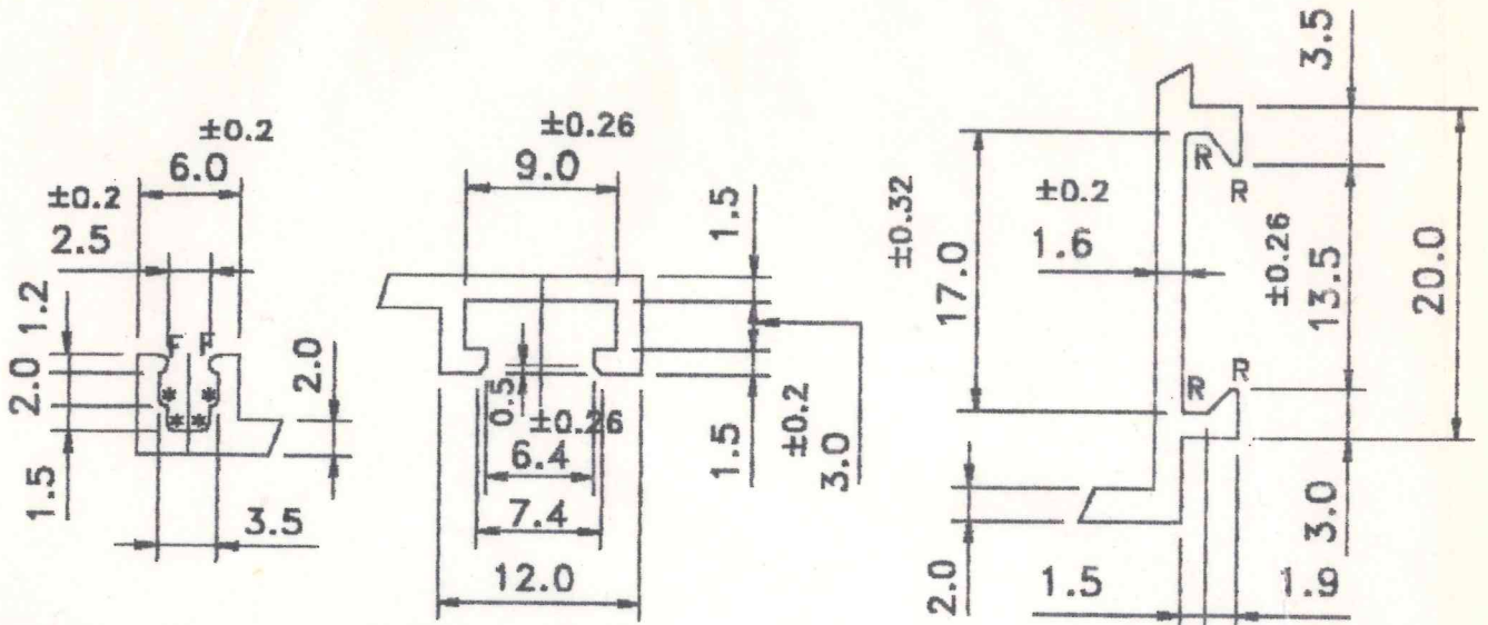
DETAIL AT = C
