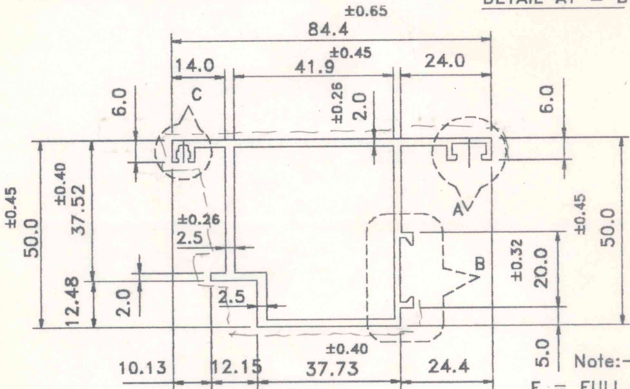
DETAIL AT = B
