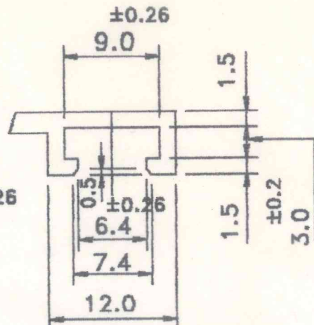
DETAIL AT = A
