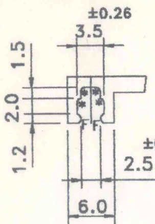
DETAIL AT = C
