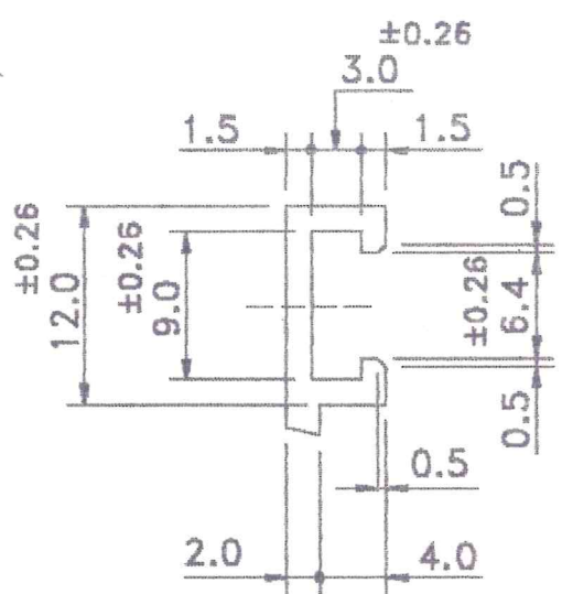
Detail At:-B
