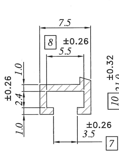
DETAIL AT-C
