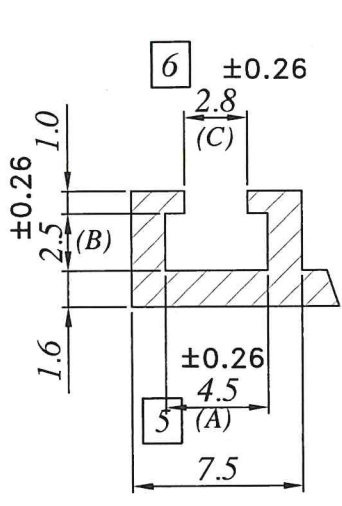
DETAIL AT-A
