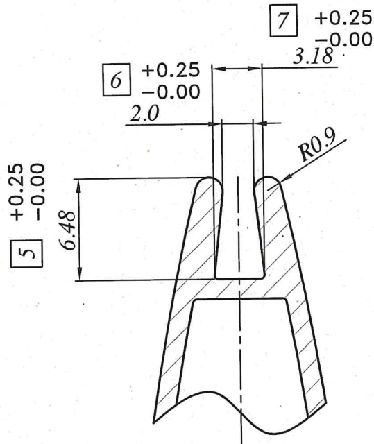
DETAIL AT- A
