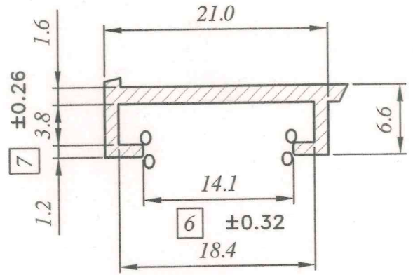
DETAIL AT- B
