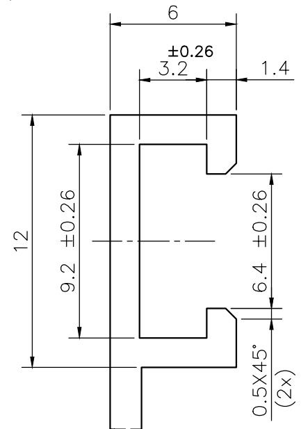
DETAIL B SCALE 4:1
