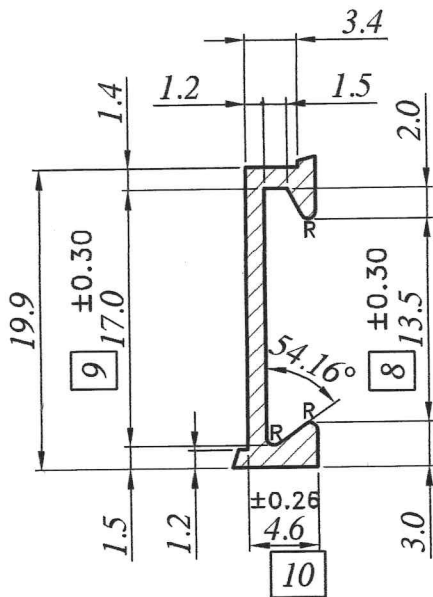
DETAIL AT- A
