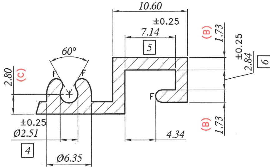
DETAIL AT- A
