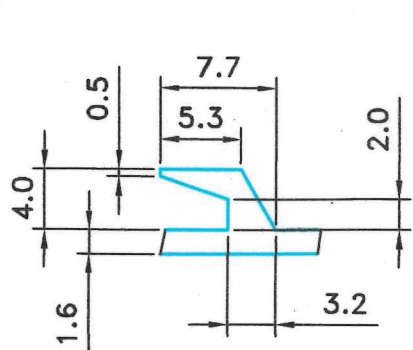
DETAIL AT = A
