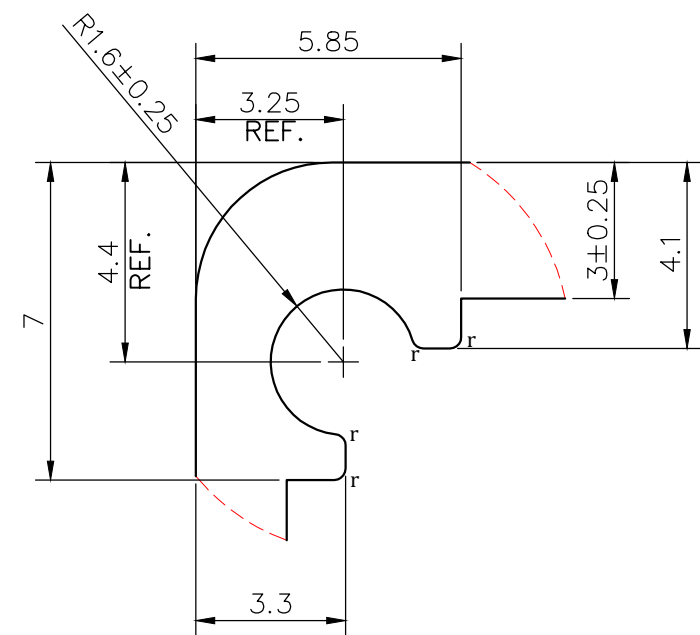
DETAIL-A SCALE 6:1
