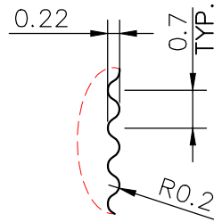
DETAIL-A SCALE 8:1
