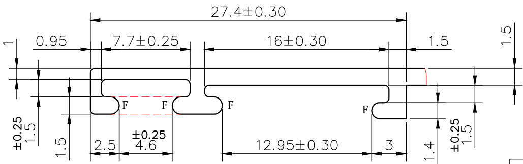
DETAIL-A SCALE 3:1
