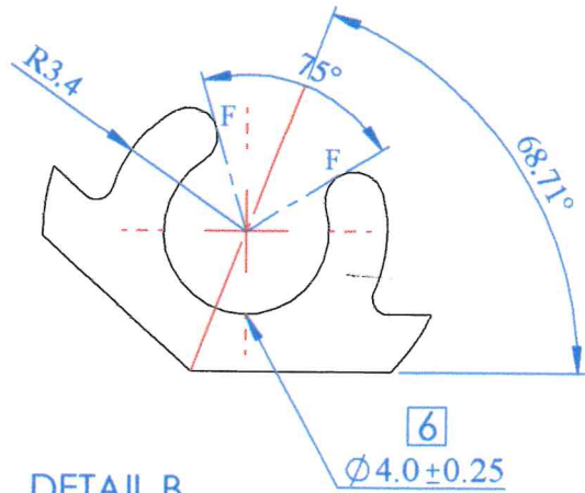
DETAIL B SCALE 5 : 1
