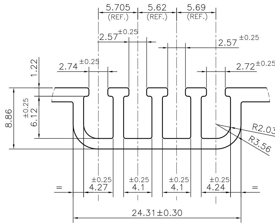
DETAIL B SCALE 3:1
