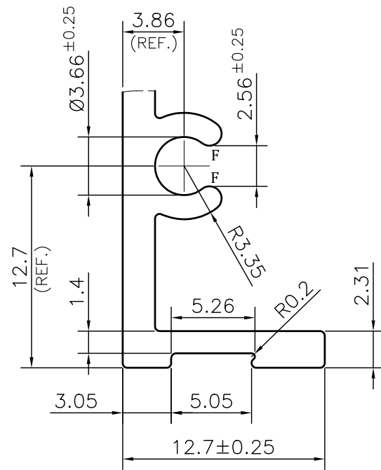
DETAIL A SCALE 3:1
