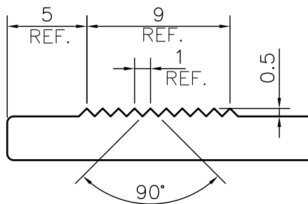
DETAIL A SCALE 3:1
