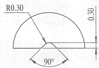
DETAIL "B" SCALE 10 : 1
