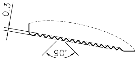
DETAIL A SCALE 4:1
