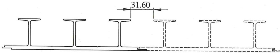
ASSEMBLY SCALE 1:3
