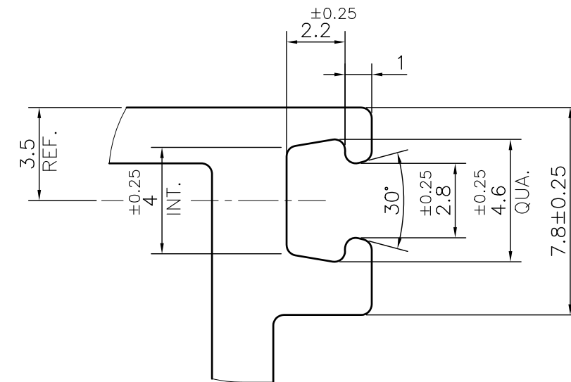
DETAIL B SCALE 5:1
