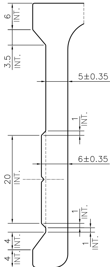
DETAIL A SCALE 2:1
