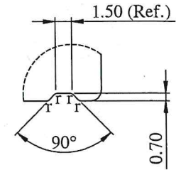
DETAIL A SCALE 3 : 1
