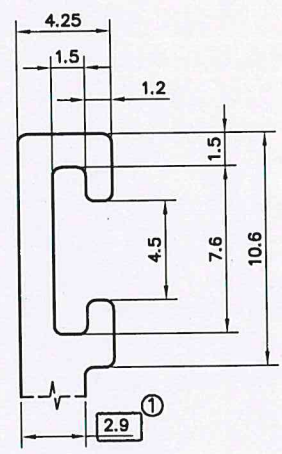
DETAIL A SCALE 4:1
