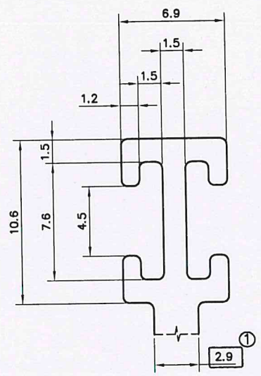
DETAIL B SCALE 4:1
