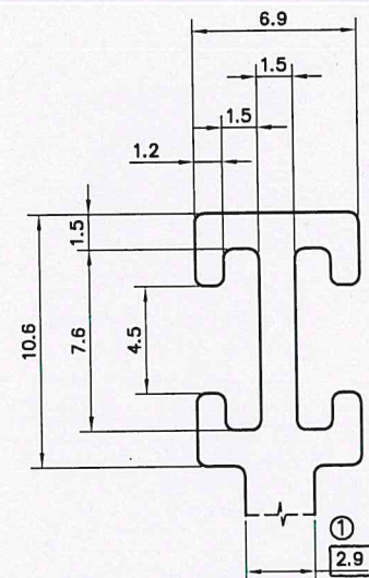
DETAIL B SCALE 4:1
