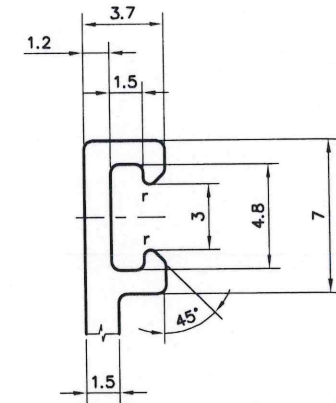
DETAIL A SCALE 4:1
