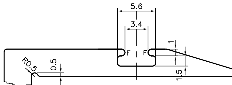
DETAIL OF "B" SCALE 3:1
