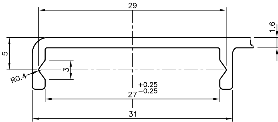
DETAIL OF "A" SCALE 3:1
