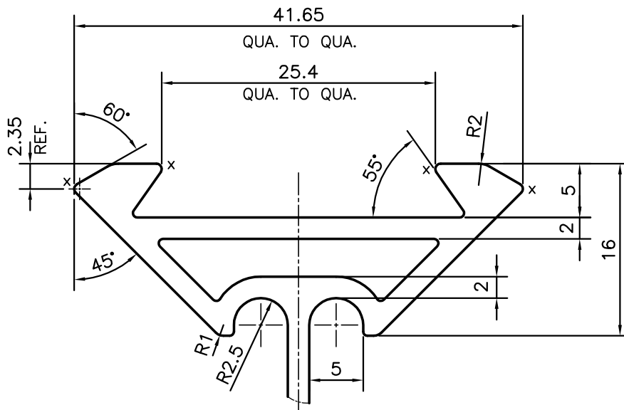
DETAIL OF "A" SCALE 2:1
