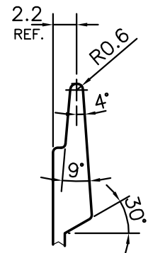
DETAIL OF "C" SCALE :- 2:1
