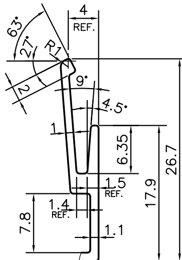
DETAIL OF "A" SCALE :- 2:1
